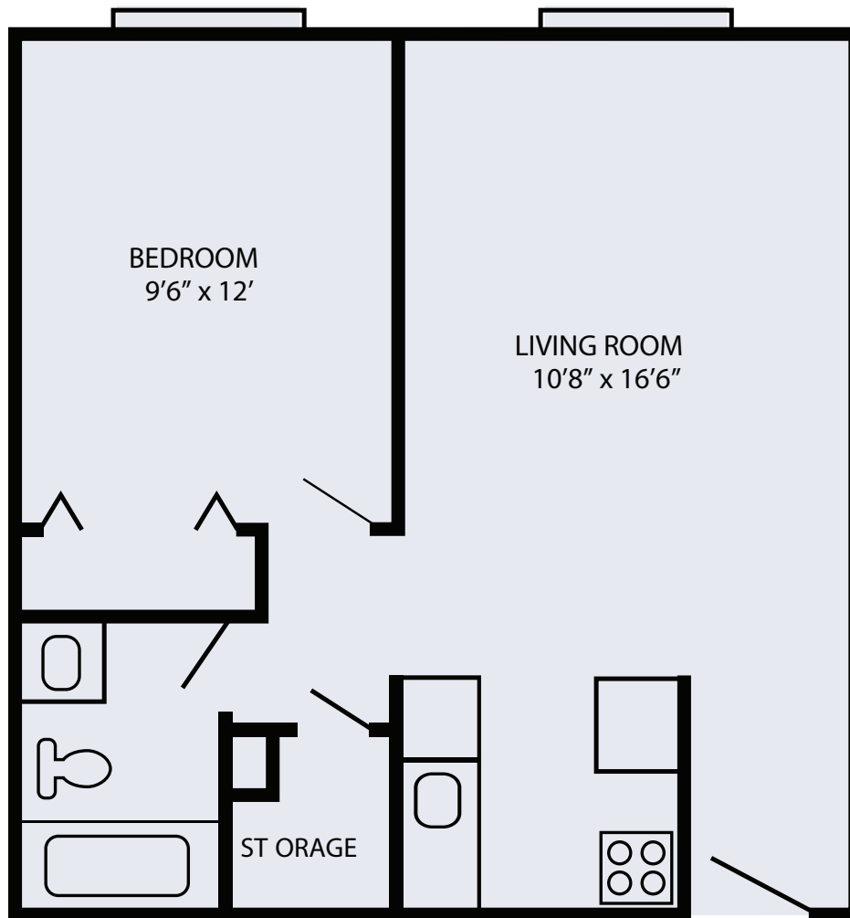
One Bedroom - Plan B 460 Square Feet
